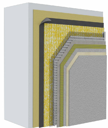
StoPowerwall® Drainscreen® with Sto Crack Defense option
